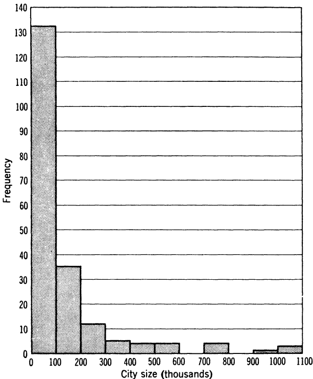
Fig. 2.1. Frequency distribution of sizes of 196 United States Cities in 1920.
