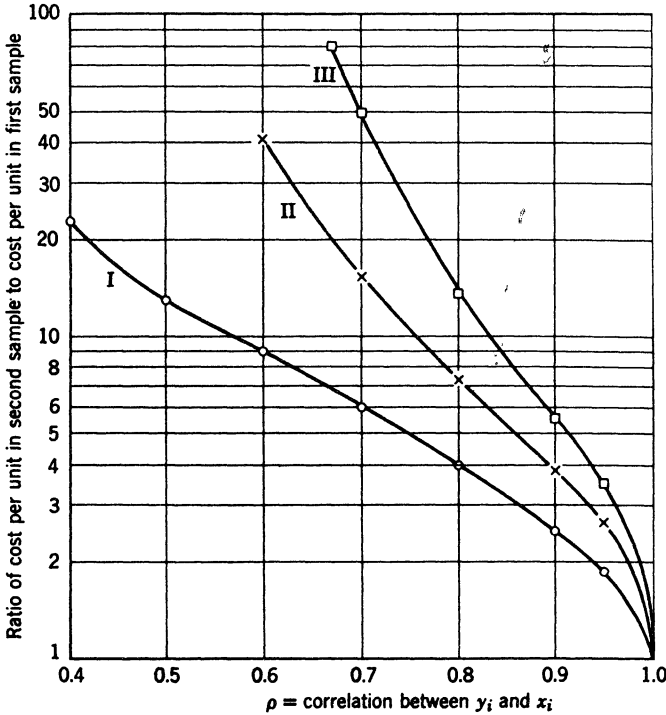
Fig. 12.1 Relation between c/c' and \rho for three fixed values of the relative precision of double and single sampling.
