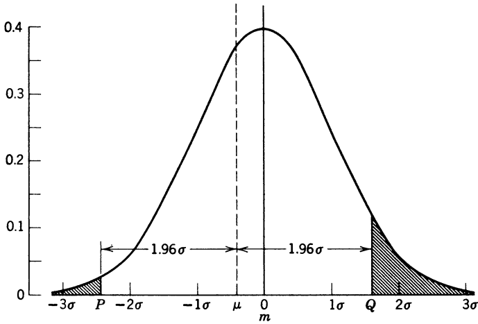
Fig. 1.1 Effect of bias on errors of estimation.
