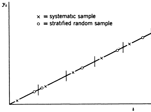
Fig. 8.2 Systematic sampling in a population with linear trend.
