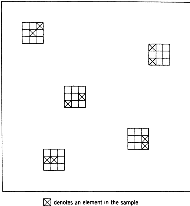
Fig. 10.1 Schematic representation of two-stage sampling ( N = 81, n = 5, M = 9, m = 2 ).
