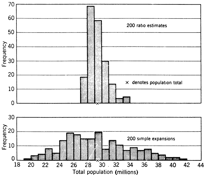
Fig. 6.1 Experimental comparison of the ratio estimate with the estimate based on the sample mean.
