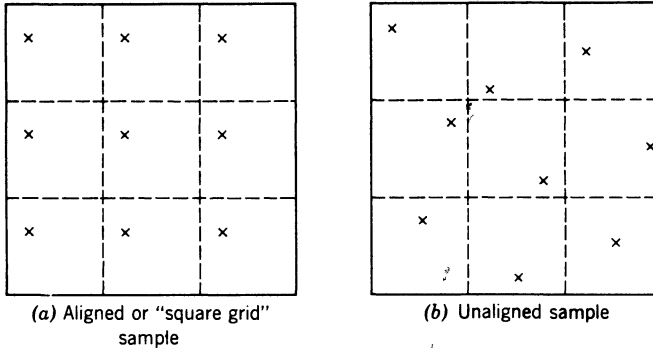
Fig. 8.4 Two types of two-dimensional systematic sample.
