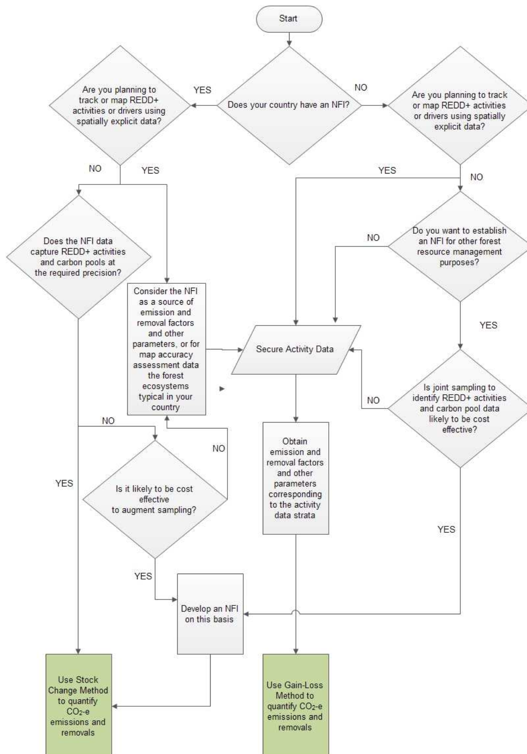
Figure 3: Decision Tree to guide selection of the method for estimating CO 2 emissions and removals depending on whether a country has an existing NFI. Note that generally an NFI will only support estimation of change in biomass C pools, and not other C pools.
